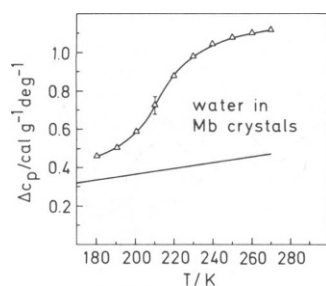
FIGURE 9 Specific heat of water in myoglobin crystals ( \Delta ) as a function of temperature. The data were calculated from the difference \Delta H/dT between two measurements. The first experiment was performed with intact crystals, the second experiment was done after drying the same crystals at 80°C under nitrogen flow in the DSC apparatus. The specific heat of bulk ice (—) is also given.
